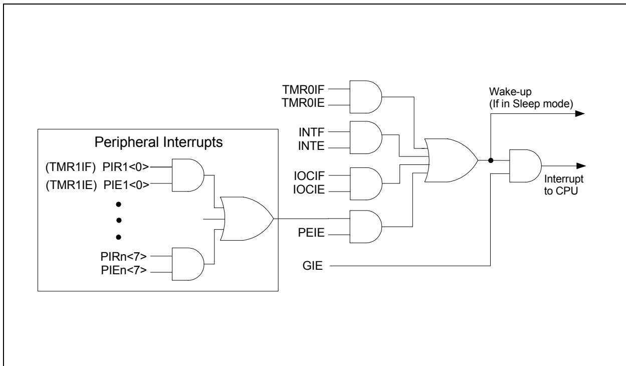
FIGURE 7-1: INTERRUPT LOGIC
