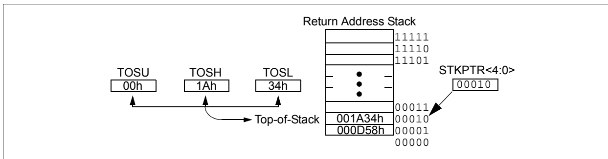
FIGURE 6-3: RETURN ADDRESS STACK AND ASSOCIATED REGISTERS
