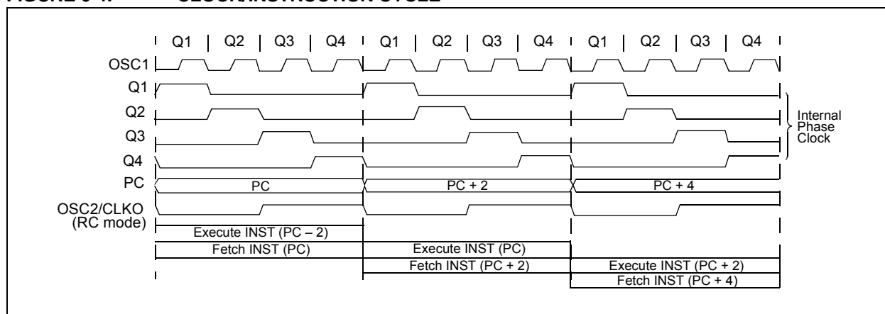
FIGURE 6-4: CLOCK/INSTRUCTION CYCLE
