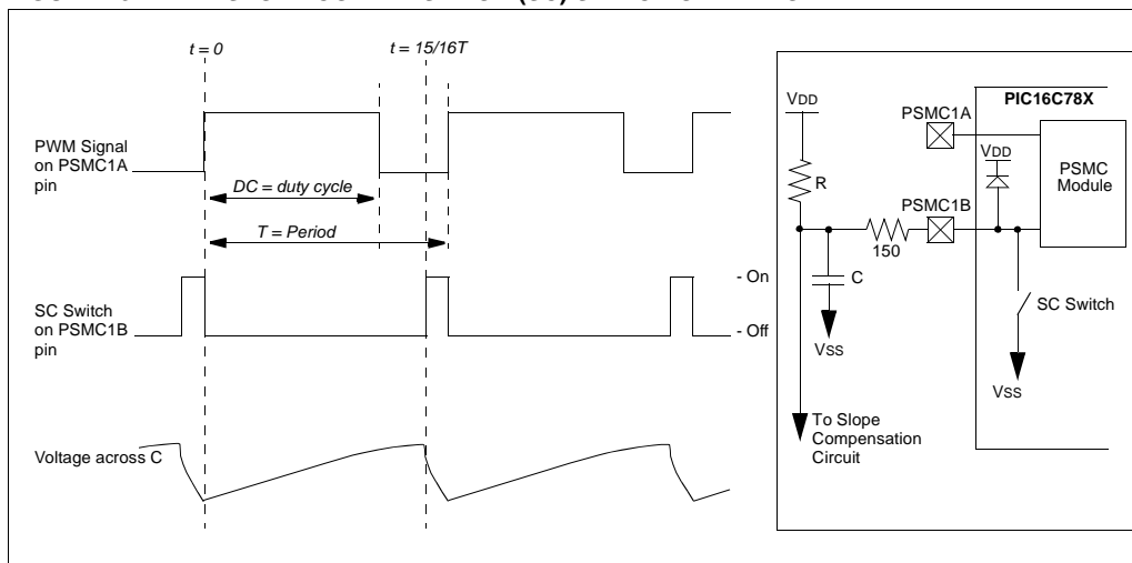
FIGURE 13-4: SLOPE COMPENSATION (SC) SWITCH OPERATION
