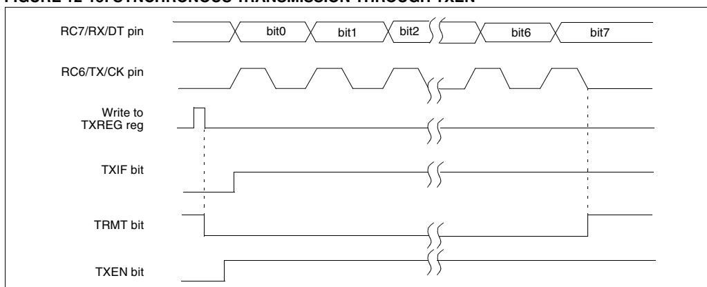
FIGURE 12-13: SYNCHRONOUS TRANSMISSION THROUGH TXEN
