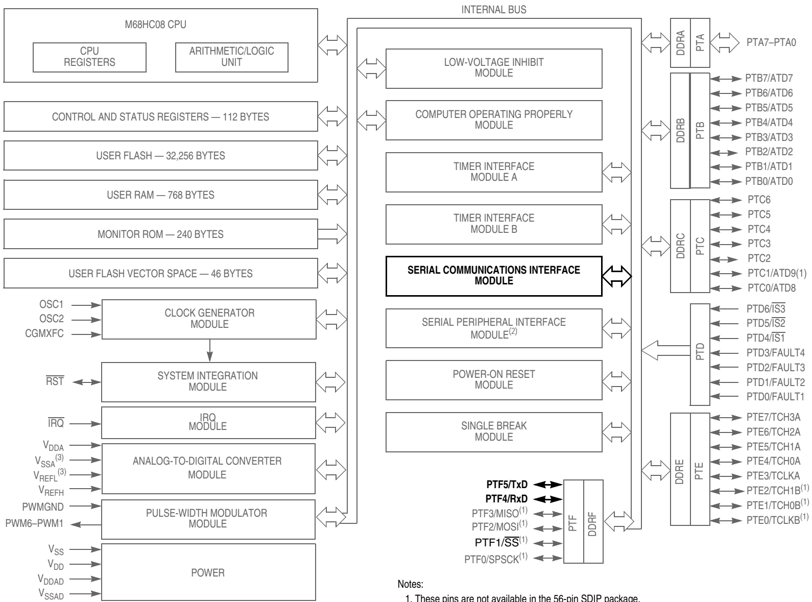
Figure 13-1. Block Diagram Highlighting SCI Block and Pins
