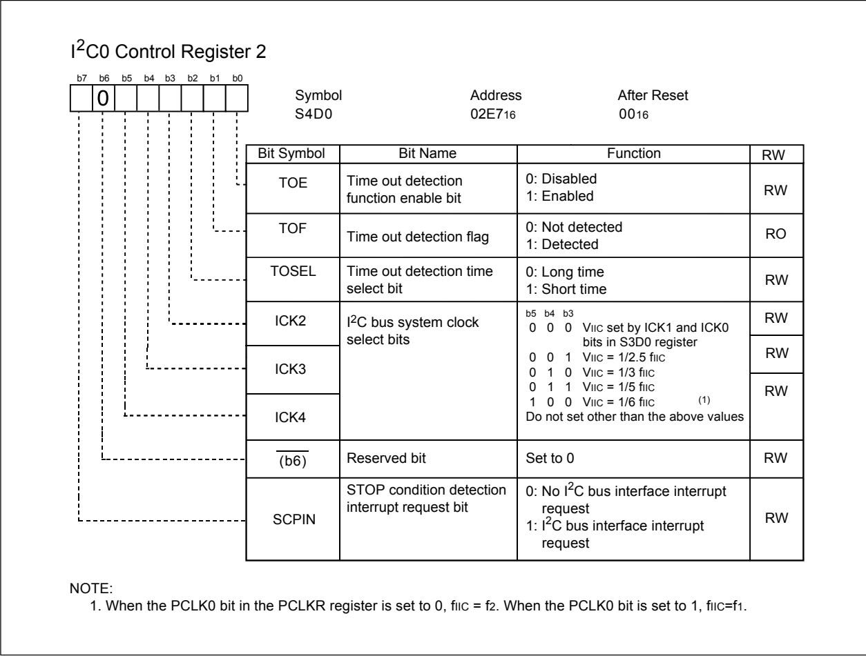
Figure 16.7 S4D0 Register
