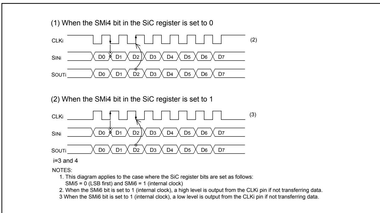
Figure 14.38 Polarity of Transfer Clock
