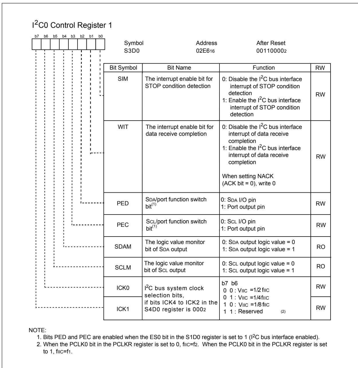
Figure 16.6 S3D0 Register
