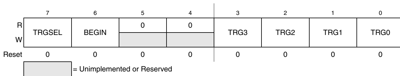
Figure 18-8. Debug Trigger Register (DBGTR)
