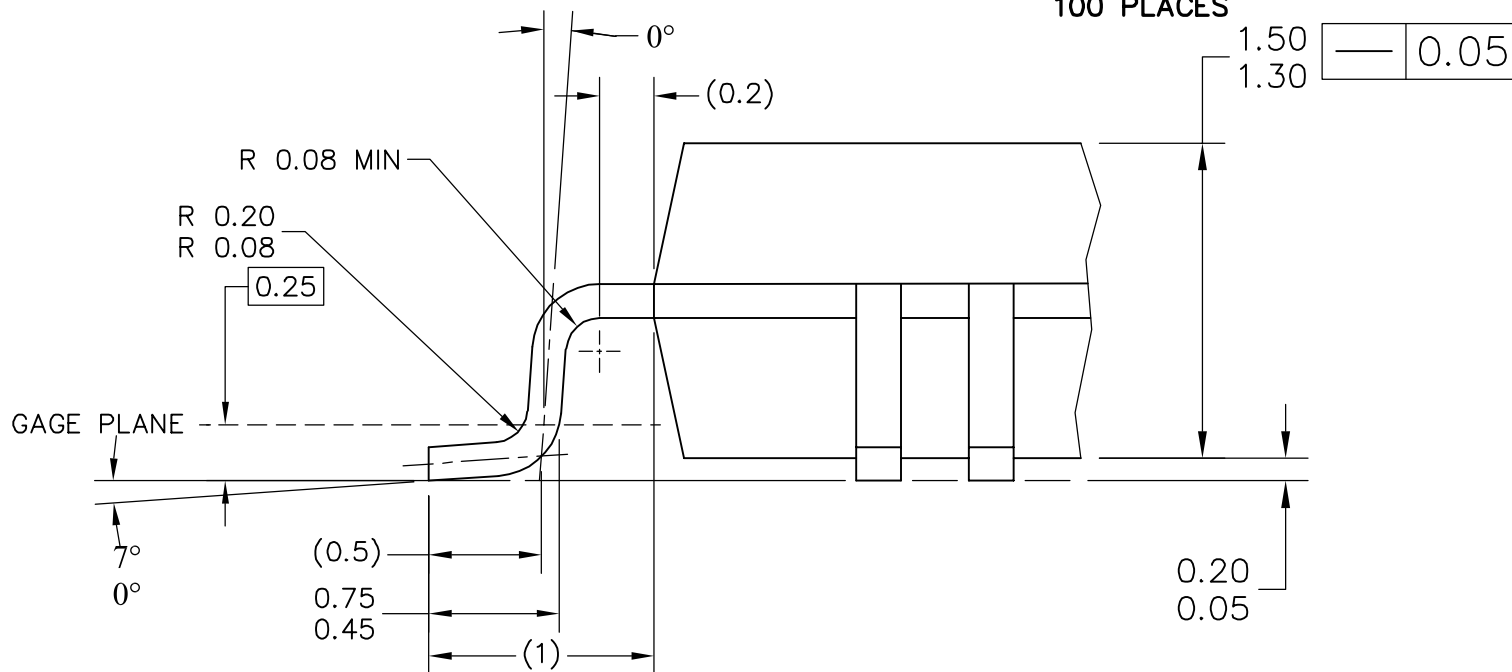
VIEW A
