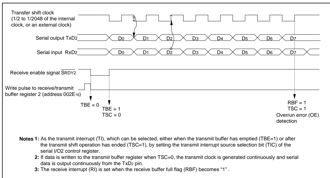
Fig. 64 Operation of clock synchronous serial I/O2 function
