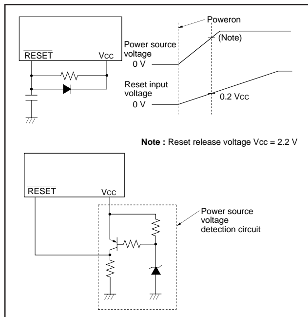
Fig. 73 Example of reset circuit
