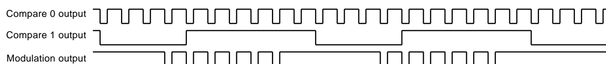
Fig. 48 Output compare mode (compare 0, 1 modulation mode: effect of output level latch)
