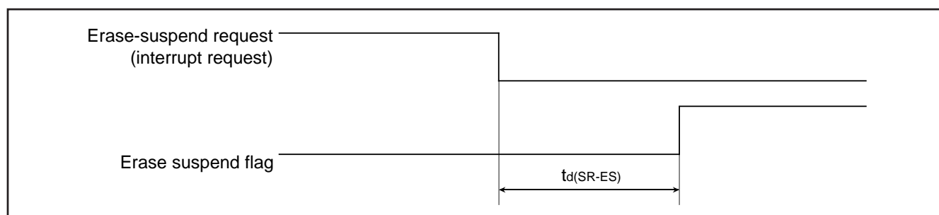
Fig. 117 Time delay from suspend request until erase suspend
