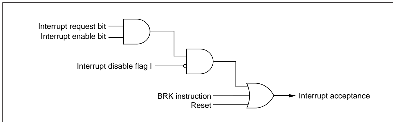
Fig. 23 Interrupt control
