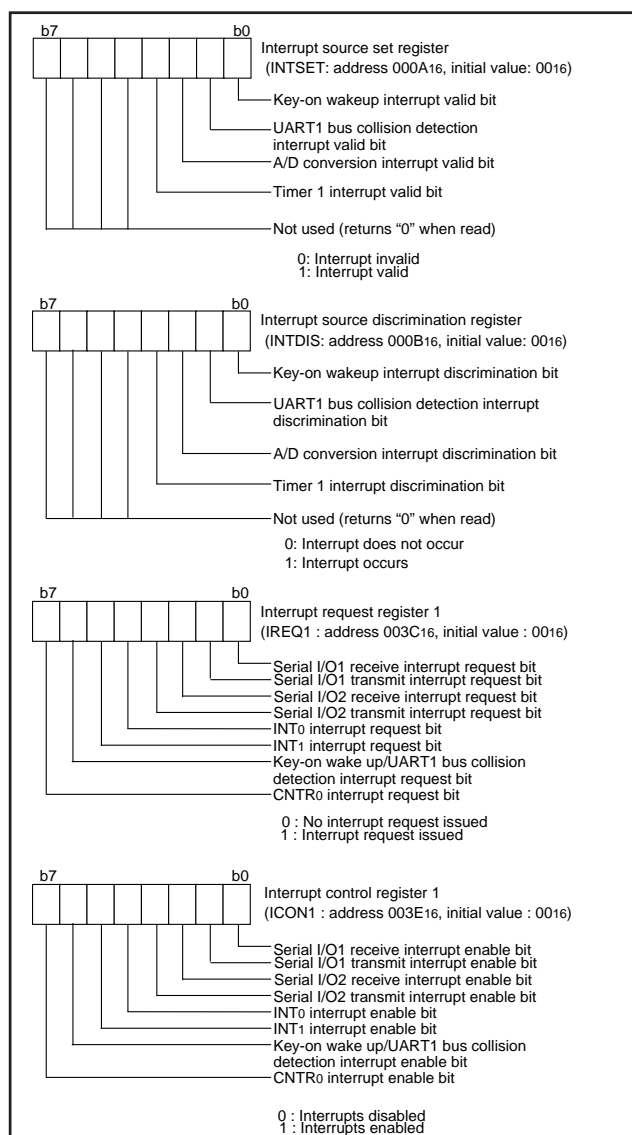
Fig. 60 Bus collision detection circuit related registers
