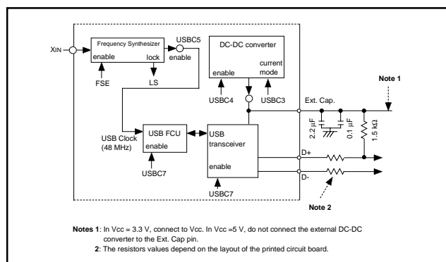
Fig.112 Peripheral circuit
