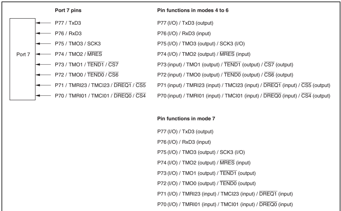
Figure 10A.4 Port 7 Pin Functions
