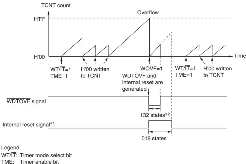
Figure 15.4 (a) WDT0 Watchdog Timer Operation
