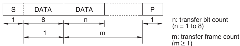
Figure 18.4 I²C Bus Data Format (Serial Format)
