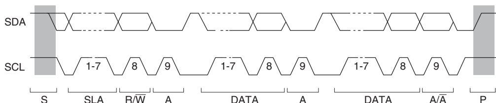
Figure 18.5 I²C Bus Timing
