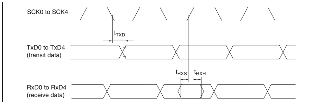
Figure 25.31 SCI Input/Output Timing (Clock Synchronous Mode)
