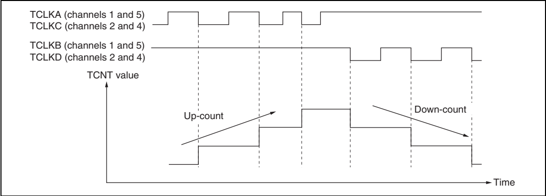
Figure 11.31 Example of Phase Counting Mode 3 Operation
