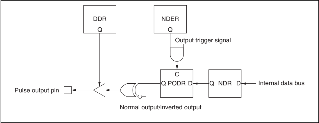
Figure 12.2 PPG Output Operation
