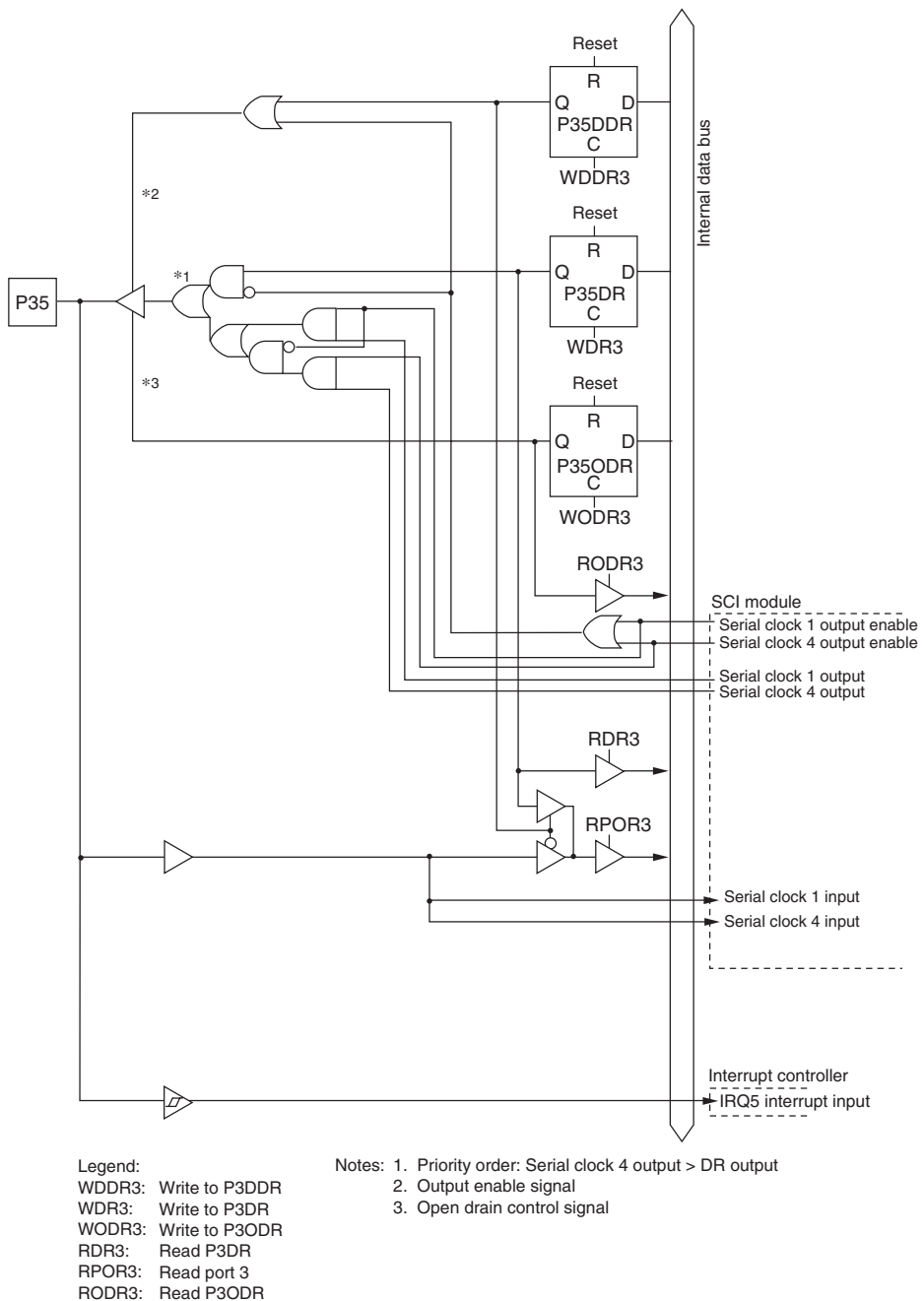
Figure C.14 (f) Port 3 Block Diagram (Pin P35)
