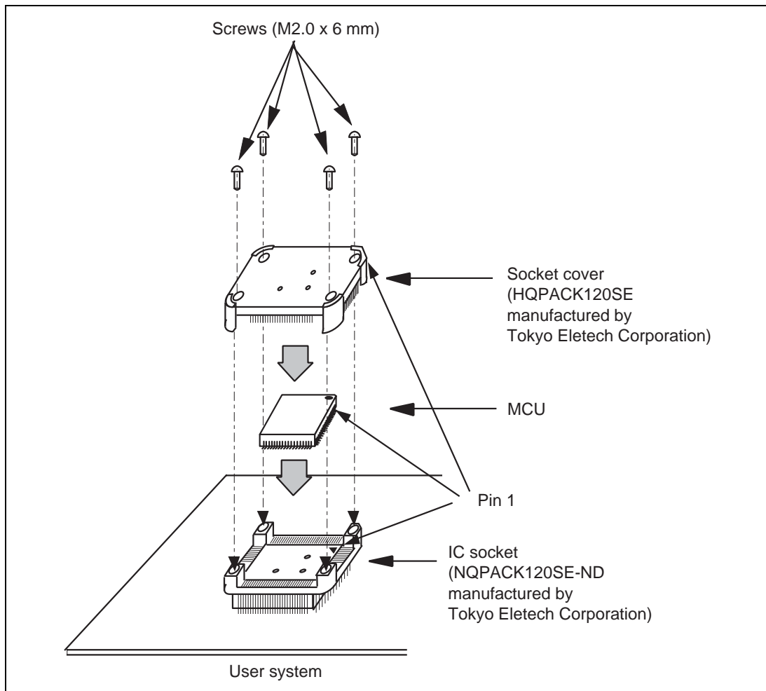
Figure 11 Installing the MCU on the User System
