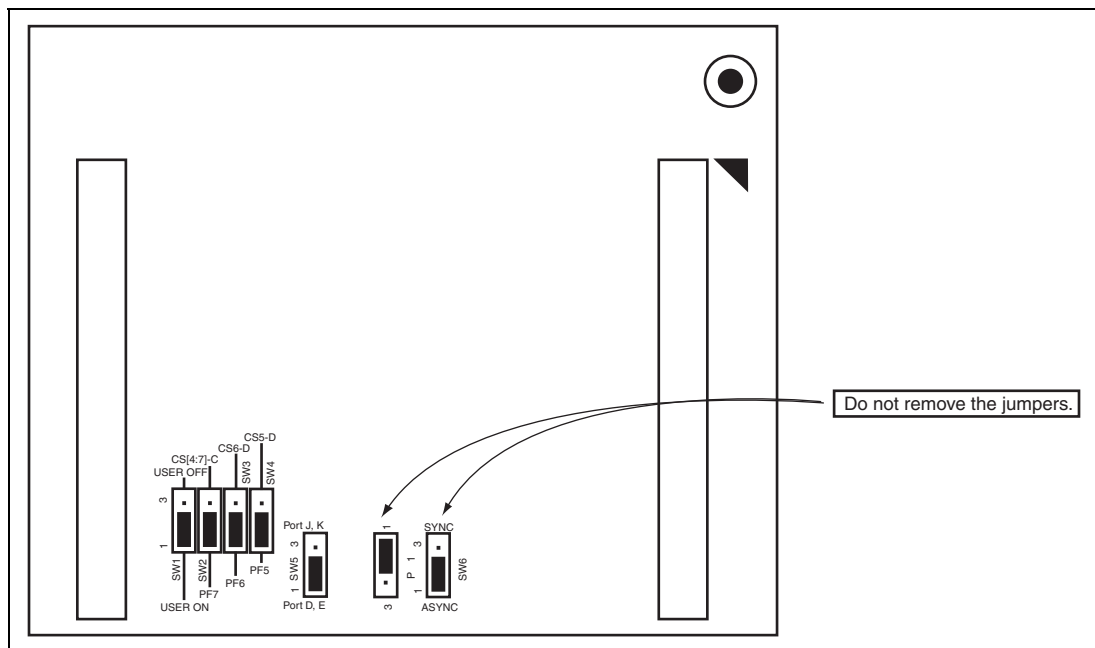
Figure 19 P1 and SW6 Jumper Sockets
