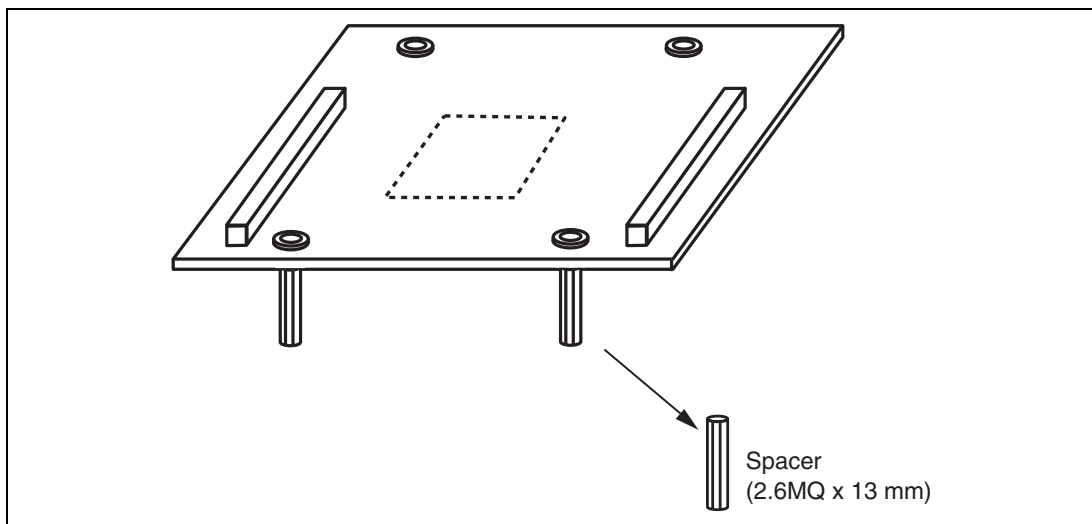
Figure 10 Attaching Spacers
