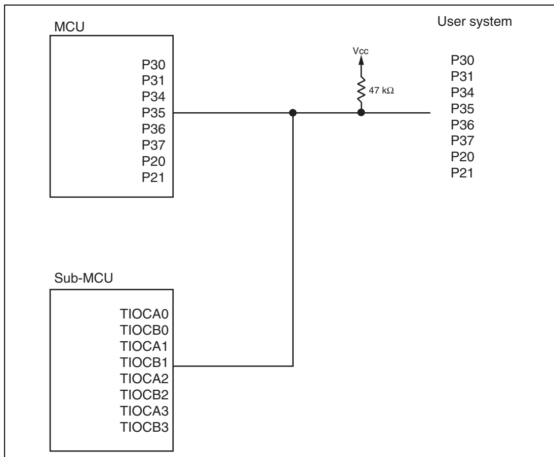
Figure 13 User System Interface Circuit (2)
