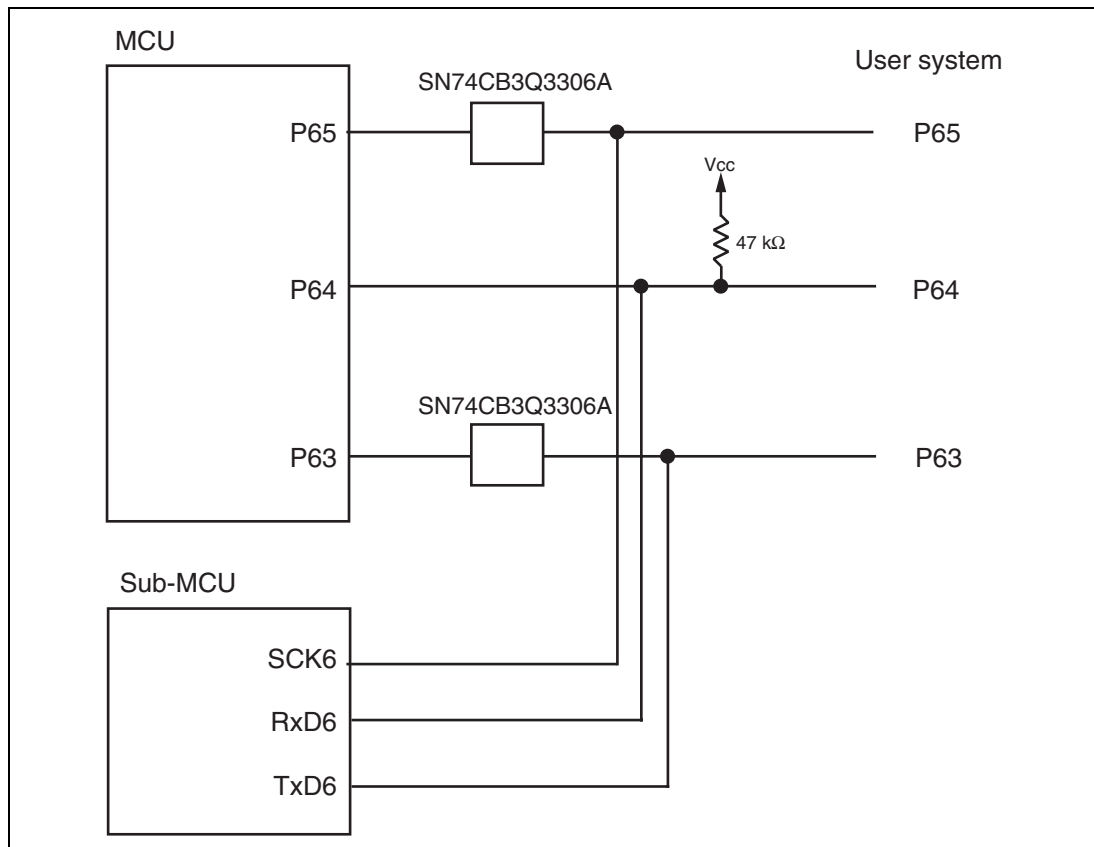
Figure 15 User System Interface Circuit (4)
