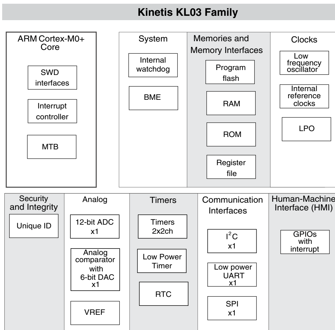
Figure 1. KL03 family block diagram
