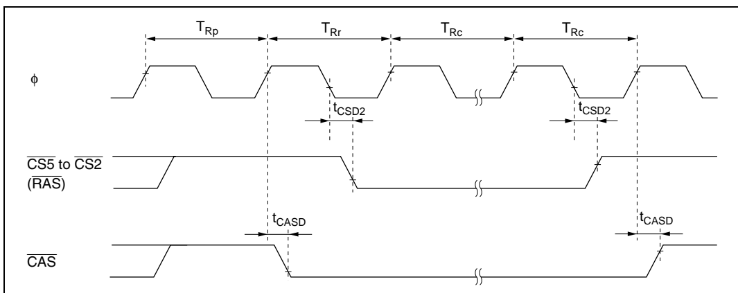
Figure 21.13 Self-Refresh Timing
