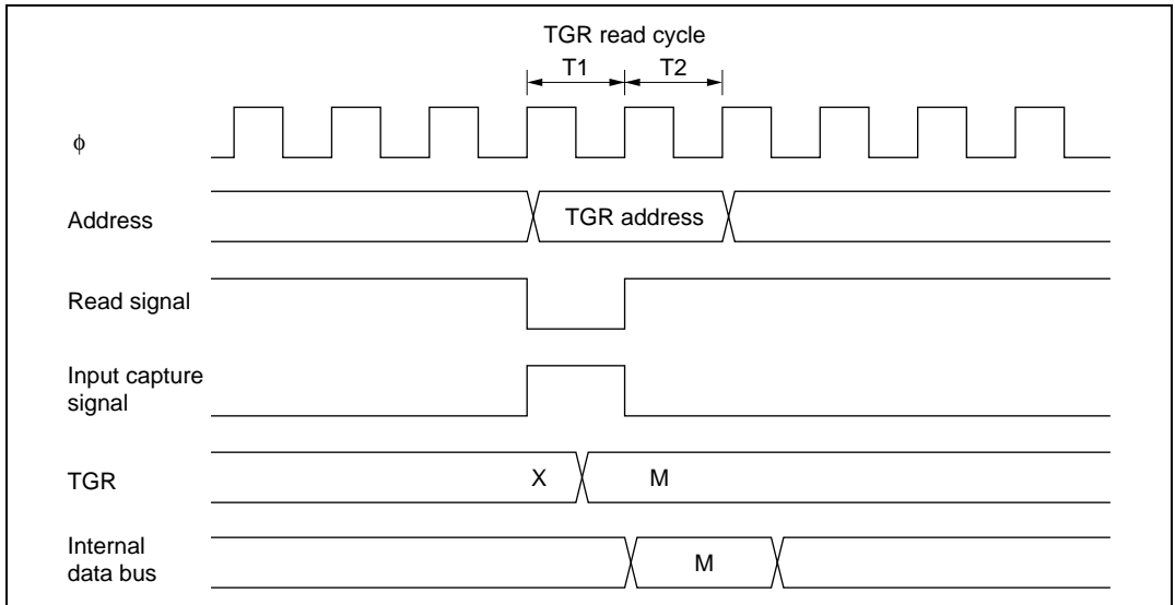
Figure 10.53 Contention between TGR Read and Input Capture
