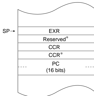
(b) Interrupt control mode 2
