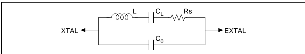
Figure 7.3 Crystal Resonator Equivalent Circuit
