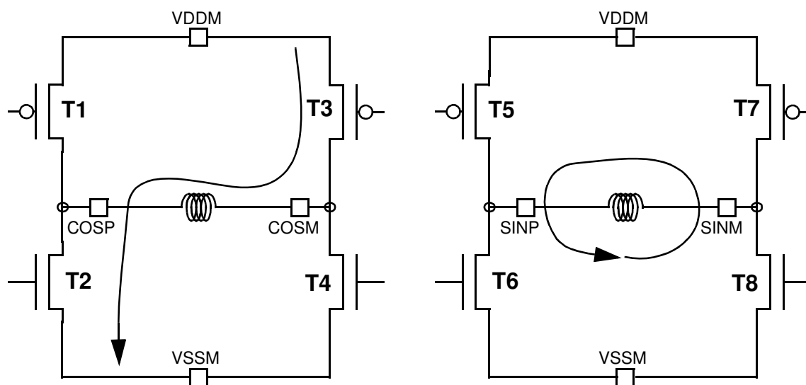
Figure 17-13. Current flow when STEP = 2, DCOIL = 1, ITG = 1
