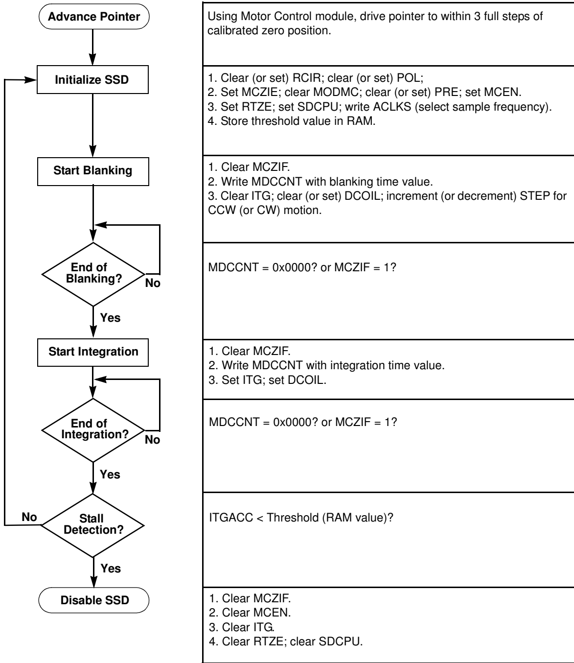
Figure 17-15. Return-to-Zero Flowchart
