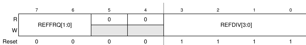
Figure 7-6. S12CPMU_UHV_V6 Reference Divider Register (CPMUREFDIV)
