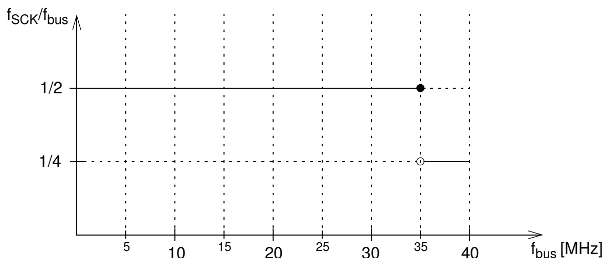
Figure M-3. Derating of maximum f_{\text{SCK}} to f_{\text{bus}} ratio in Master Mode
