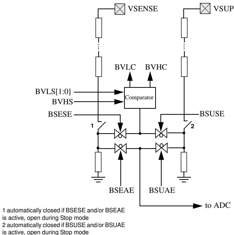
Figure 23-1. BATS Block Diagram
