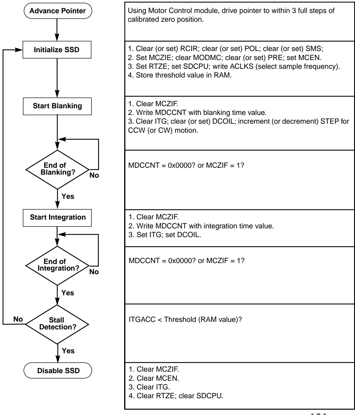
Figure 21-15. Return-to-Zero Flowchart
