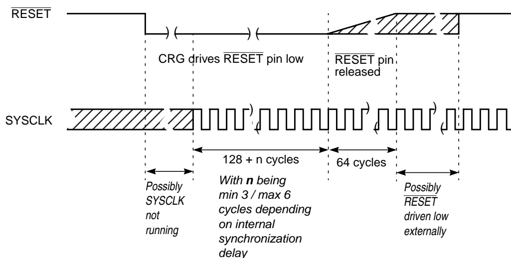
Figure 7-25. RESET Timing
