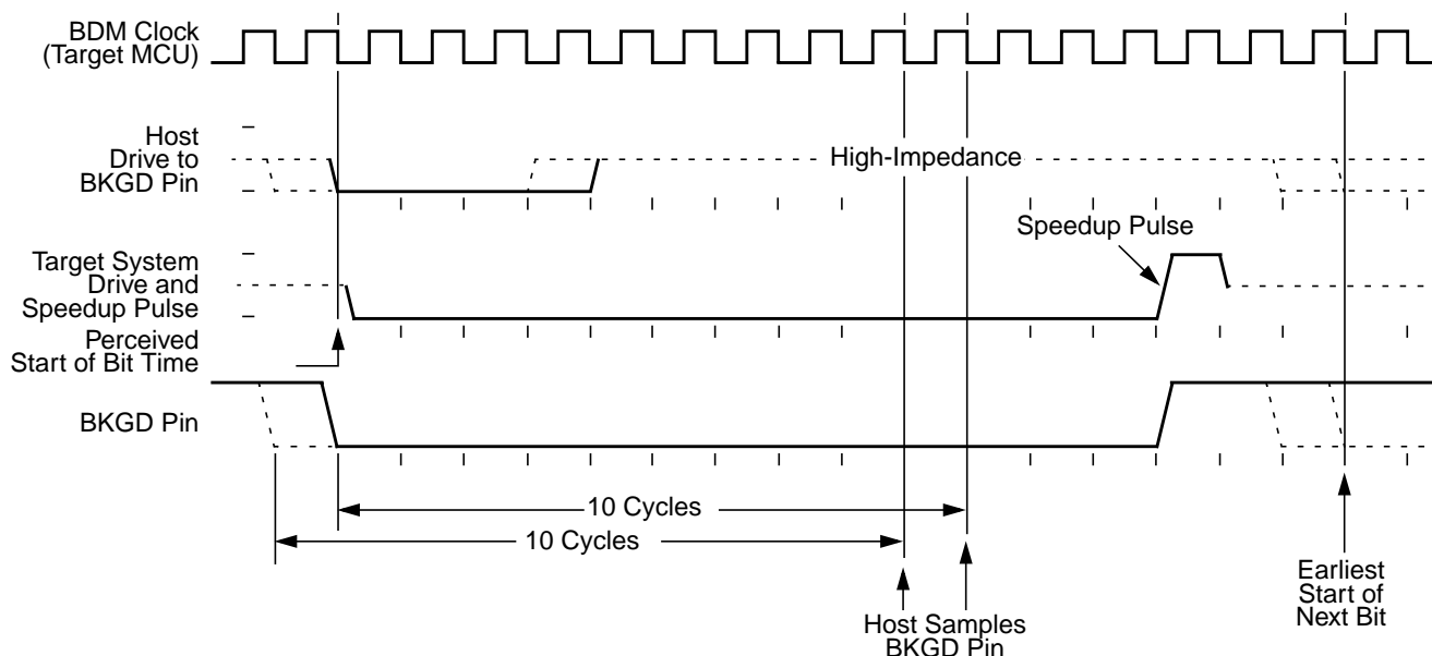
Figure 21-10. BDM Target-to-Host Serial Bit Timing (Logic 0)
