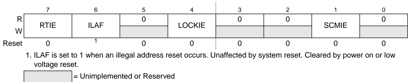
Figure 7-8. CRG Interrupt Enable Register (CRGINT)
