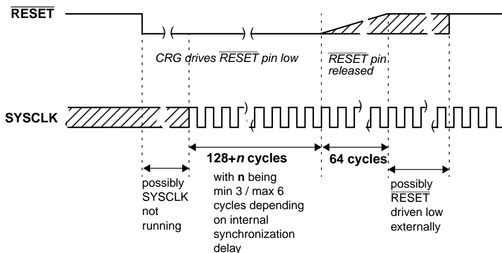
Figure 6-25. \overline{\text{RESET}} Timing
