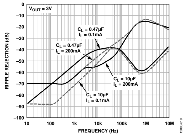
Figure 19. Power Supply Ripple Rejection vs. Frequency
