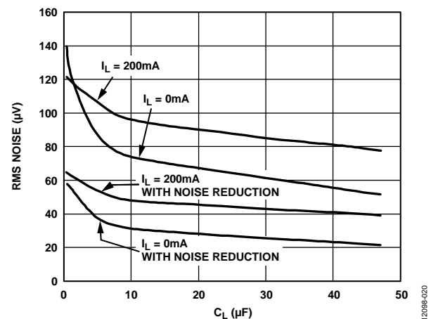
Figure 20. RMS Noise vs. C_L (10 Hz to 100 kHz)
