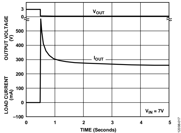
Figure 17. Short-Circuit Current
