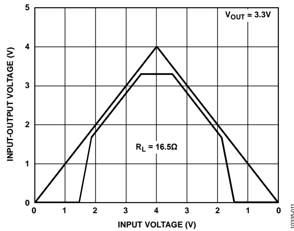
Figure 11. Power-Up/Power-Down
