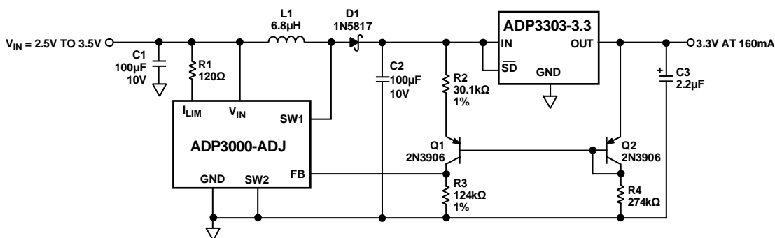
Figure 27. Constant Dropout Post Regulator
