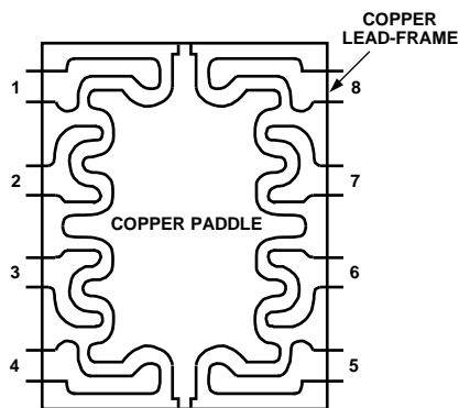
Figure 24. Thermal Coastline
