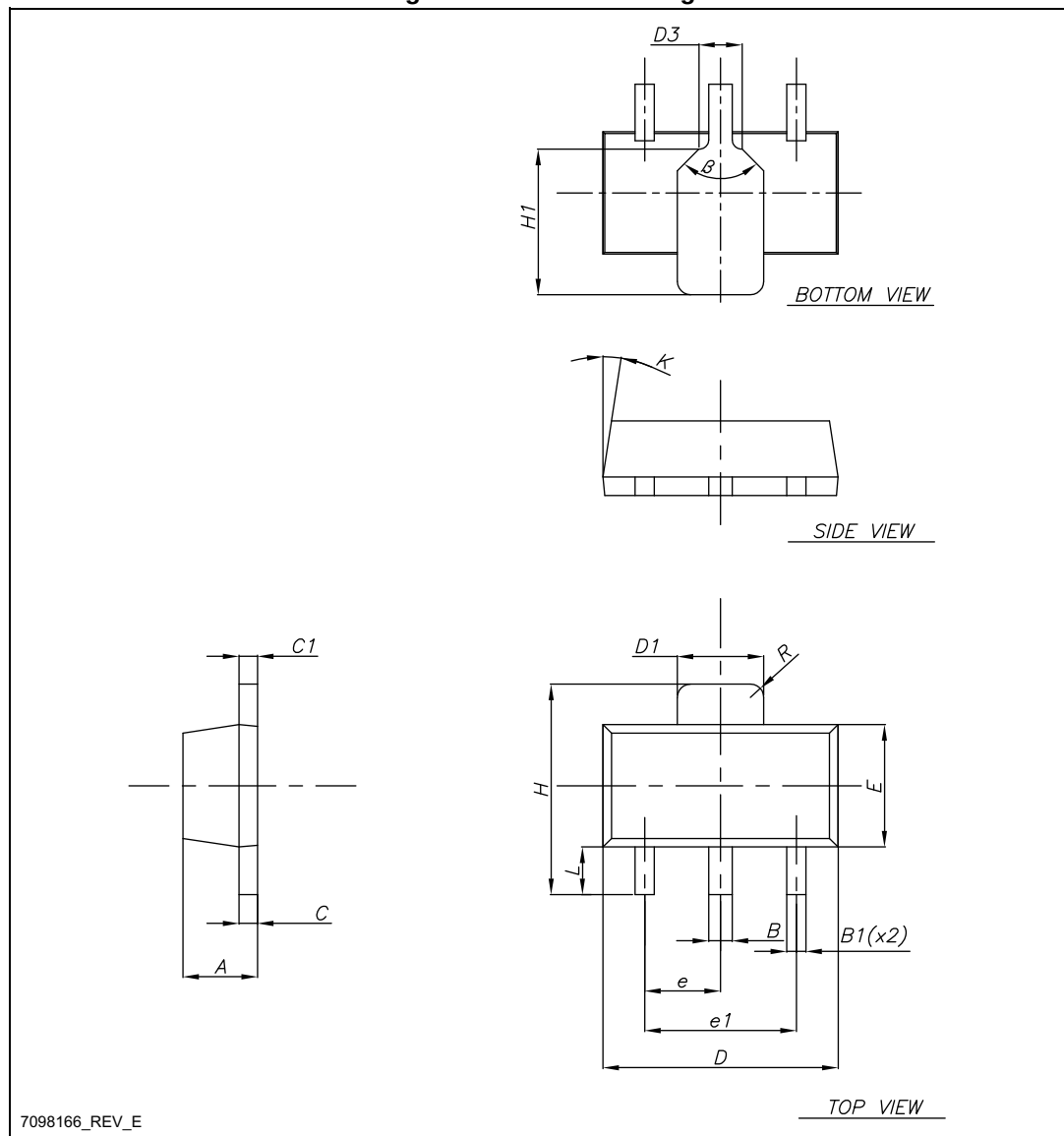
Figure 7. SOT-89 drawing
