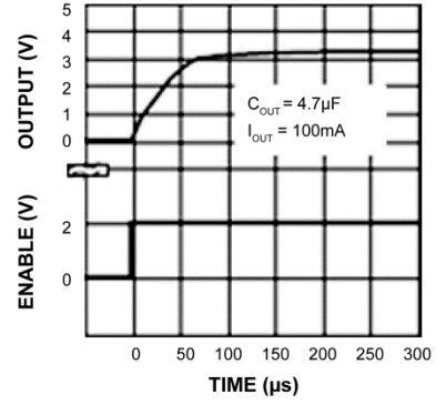
Enable Transient (3.3V Version)
