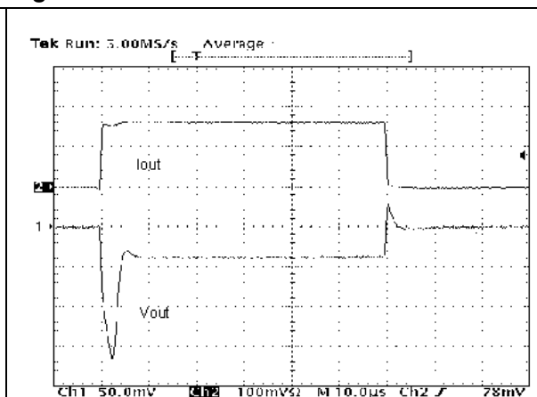
Figure 16. Load transient
