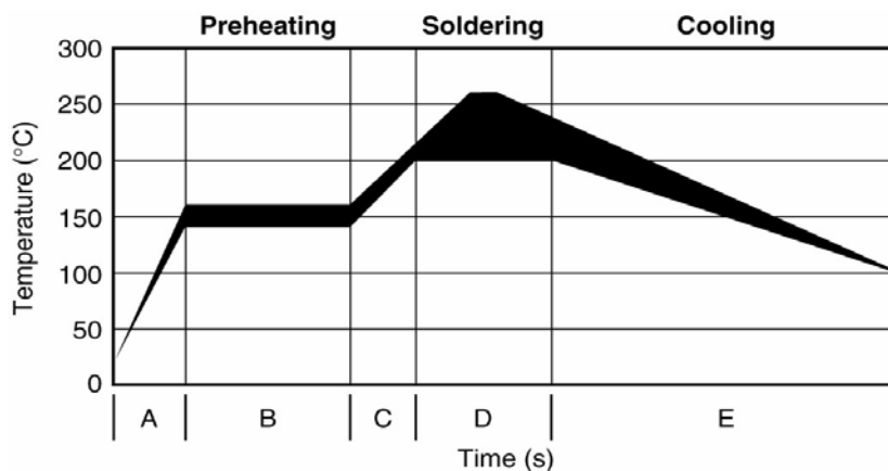
FIGURE 3. REFLOW PROFILE
