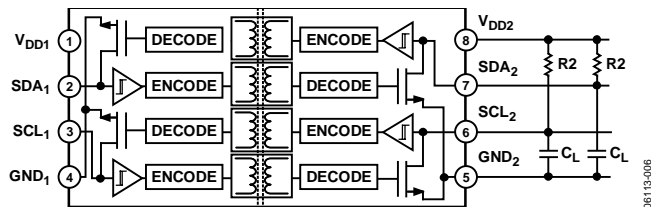
Figure 6. ADuM1250 Block Diagram
