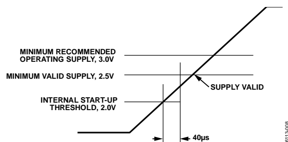
Figure 8. Start-Up Condition, Supply Slew Rate < 12.5 V/ms
