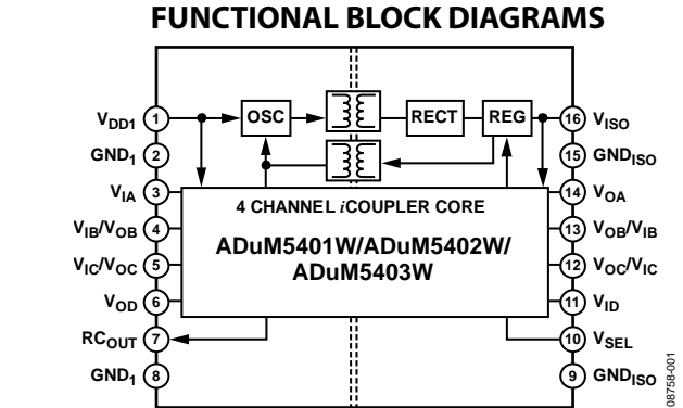
Figure 1. ADuM5401W/ADuM5402W/ADuM5403W Block Diagram
