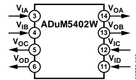
Figure 3. ADuM5402W
