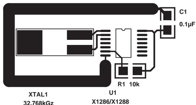
Figure 15. Suggested Layout for Intersil RTC in SO-8
