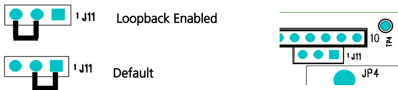
Figure 5: J11 Settings
