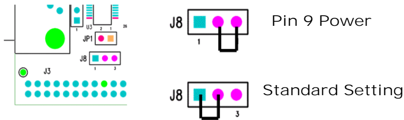
Figure 3: J8 Settings
