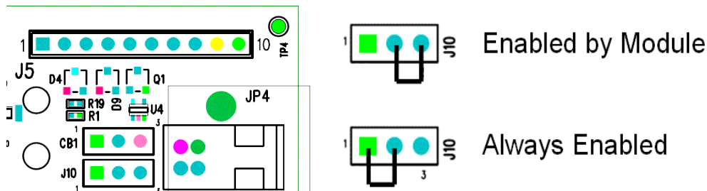
Figure 4: J10 Settings
