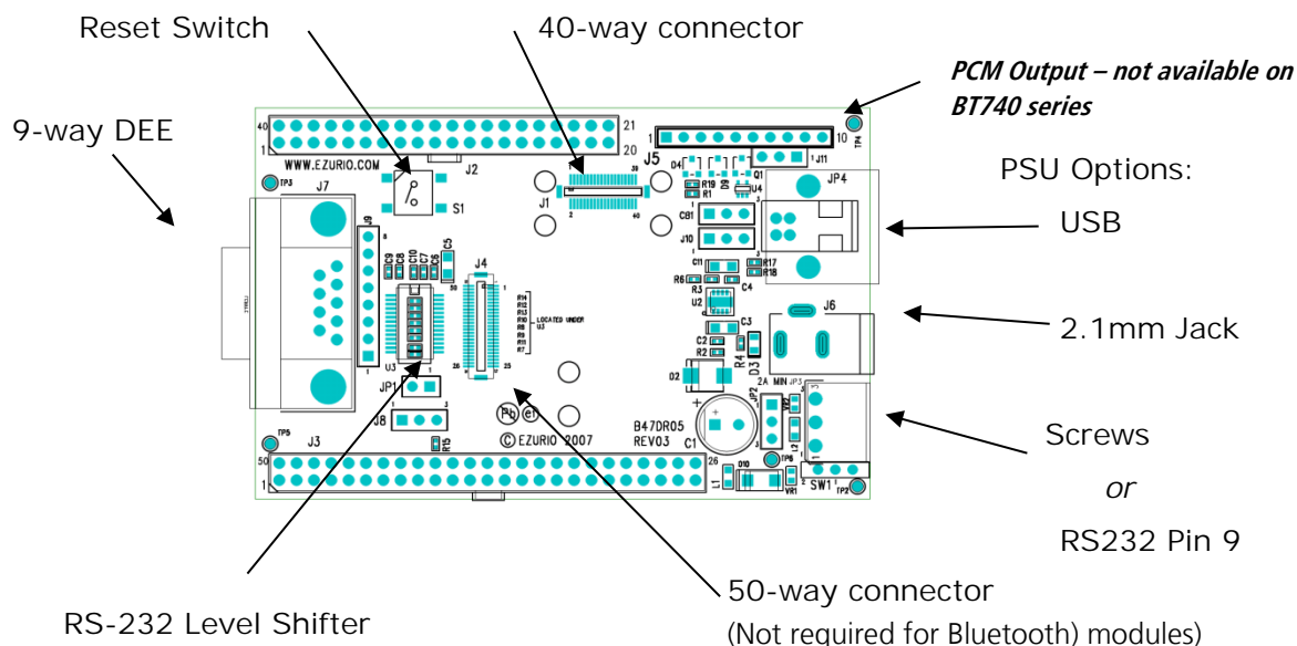
Figure 1: Development Board
