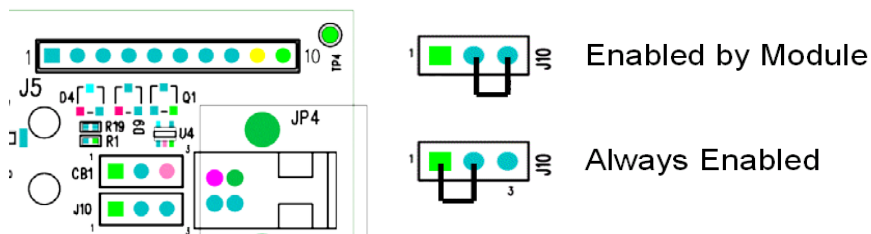
Figure 4: J10 Settings
