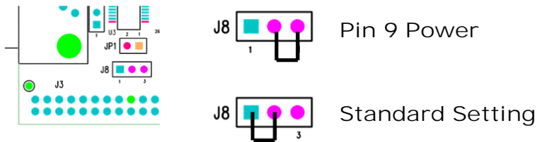
Figure 3: J8 Settings
