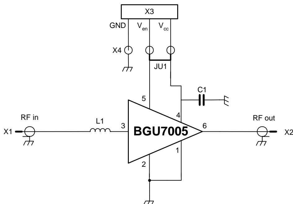
Fig 2. Circuit diagram of the BGU7005 evaluation board
