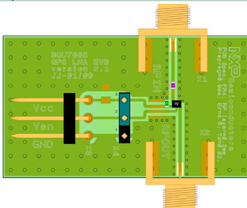
Fig 3. Printed circuit board lay-out of the BGU7005 GPS LNA evaluation board
