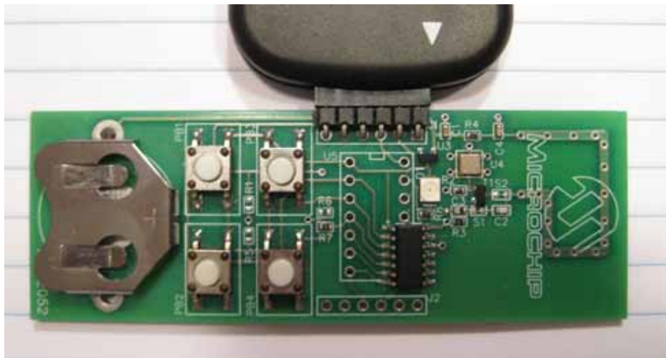
FIGURE 1-3: TRANSMITTER BOARD
