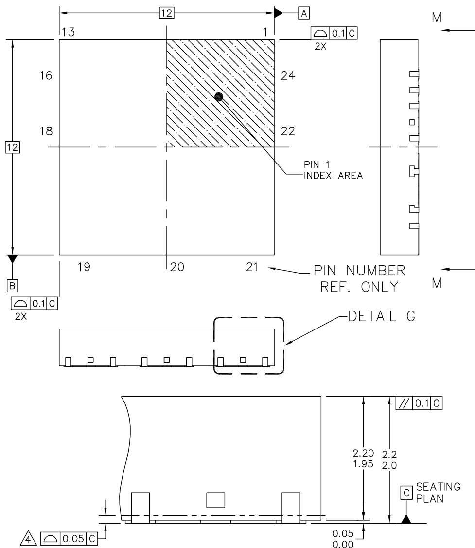
DETAIL G
