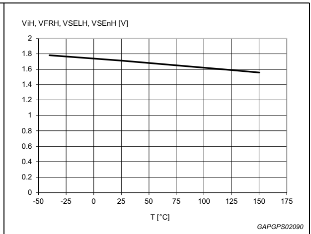
Figure 18. Logic Input high level voltage
