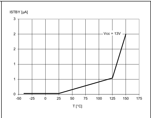
Figure 16. Standby current
