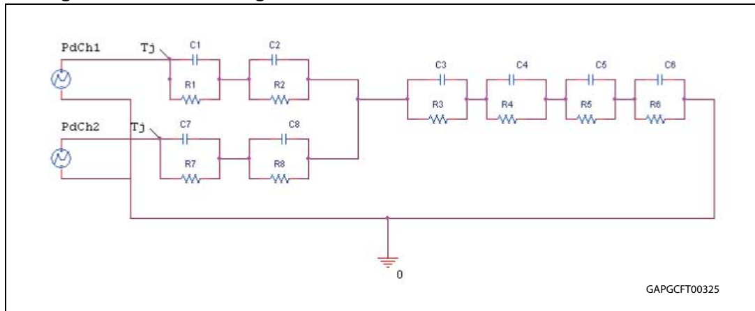
Figure 47. Thermal fitting model of a double-channel HSD in PowerSSO-16 (1)
