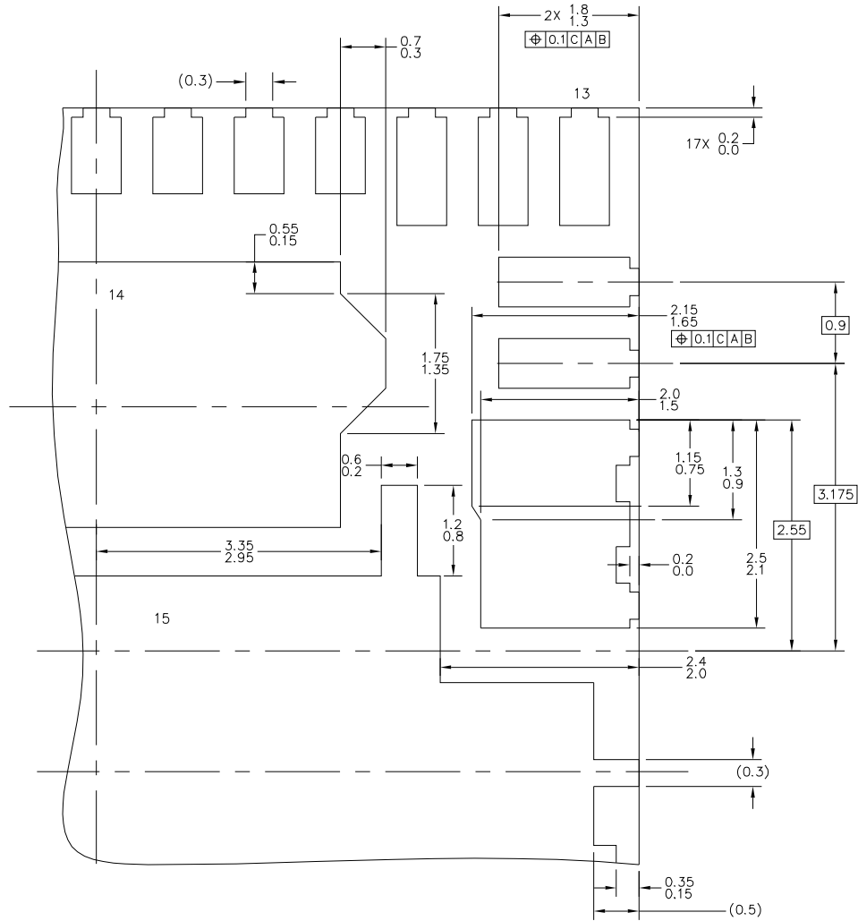
DETAIL H
