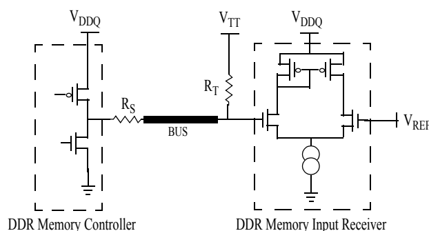
Figure 4. DDR System Level Diagram
