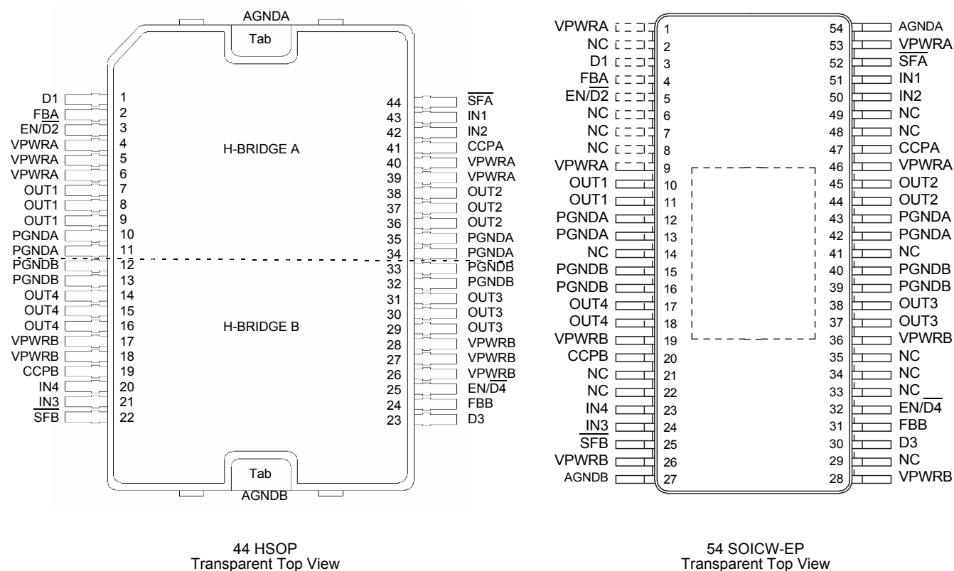
Figure 3. 33932 Pin Connections
