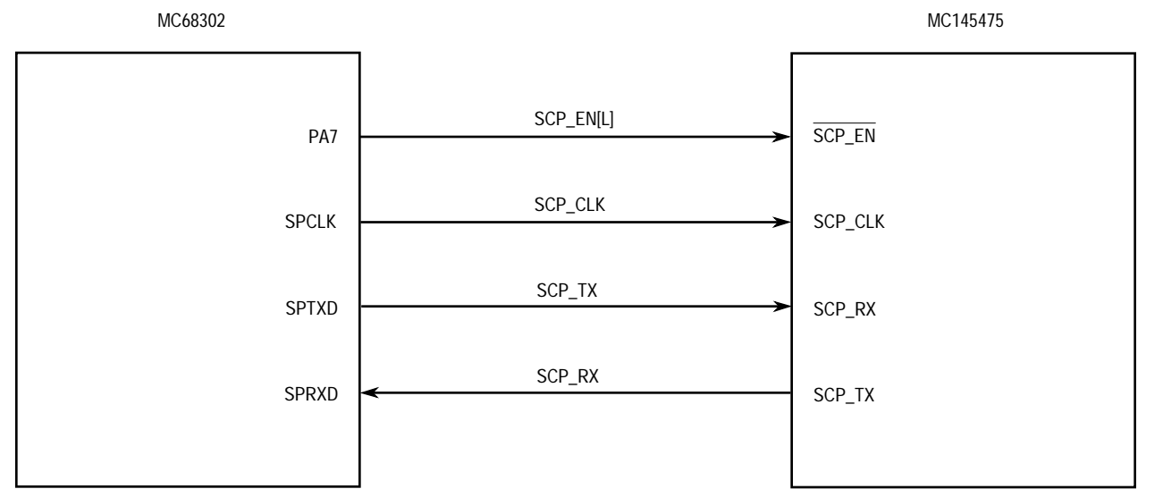
Figure D-16. SCP Bus Interconnection
