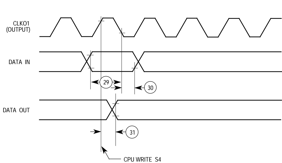
Figure 10-55. Parallel I/O Data-in/Data-Out Timing Diagram
