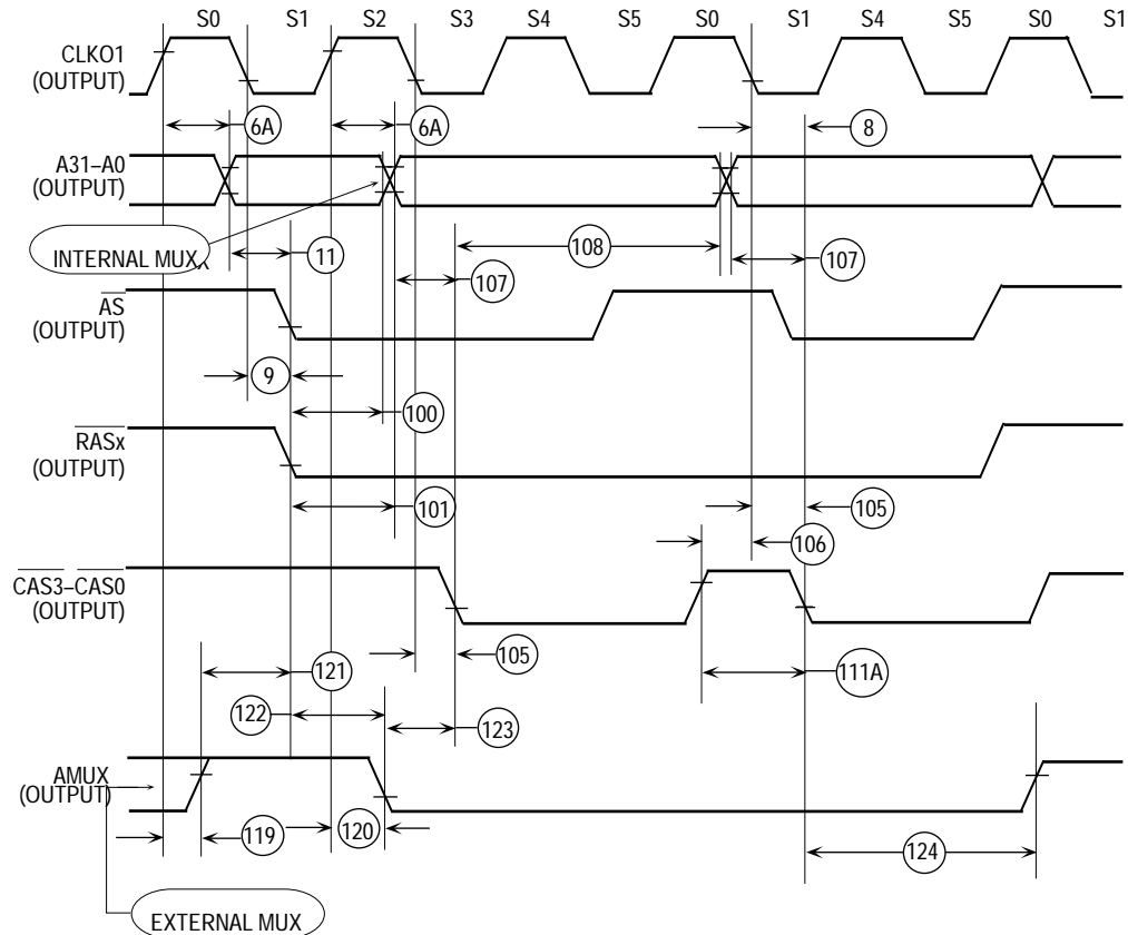
Figure 10-23. DRAM: Page-Mode—Page-Hit
