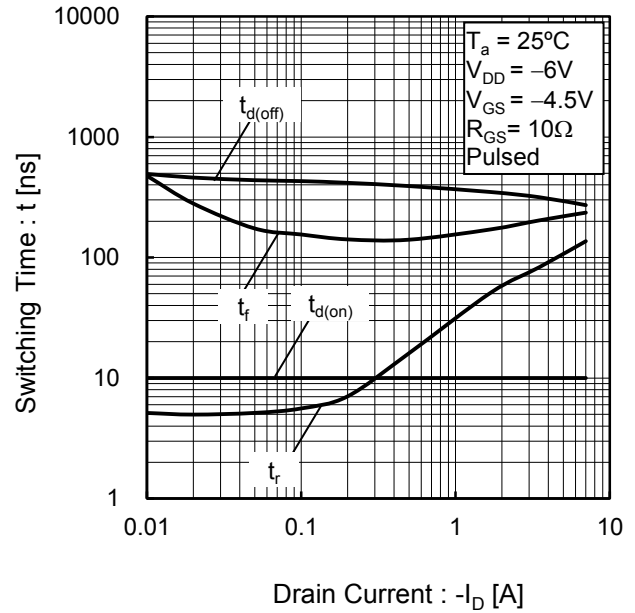
Fig.20 Switching Characteristics
