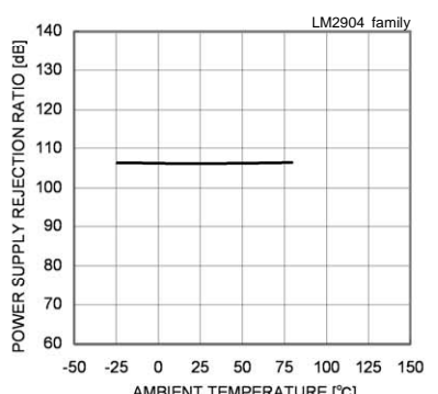
Fig. 72 Power Supply Rejection Ratio – Ambient Temperature
