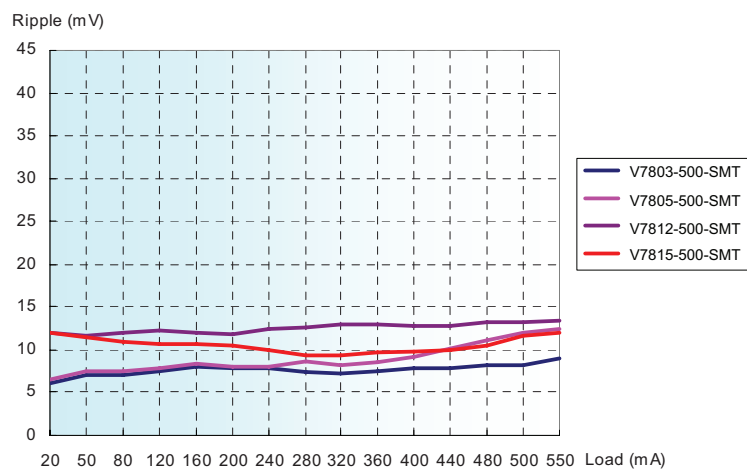
Output Voltage Ripple VS Output Load ( V_{in} =Norm)
