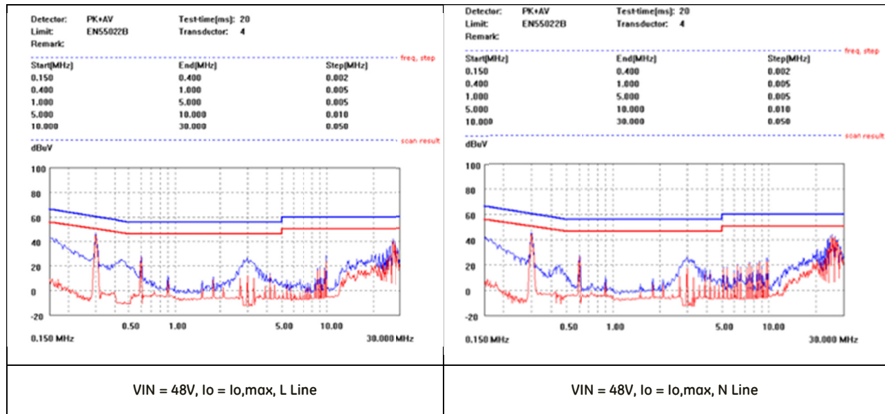
Figure 27. EMC Considerations
