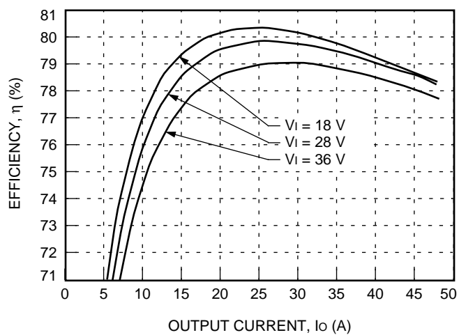
Figure 3. Typical FC250F1 Efficiency vs. Output Current at Room Temperature
