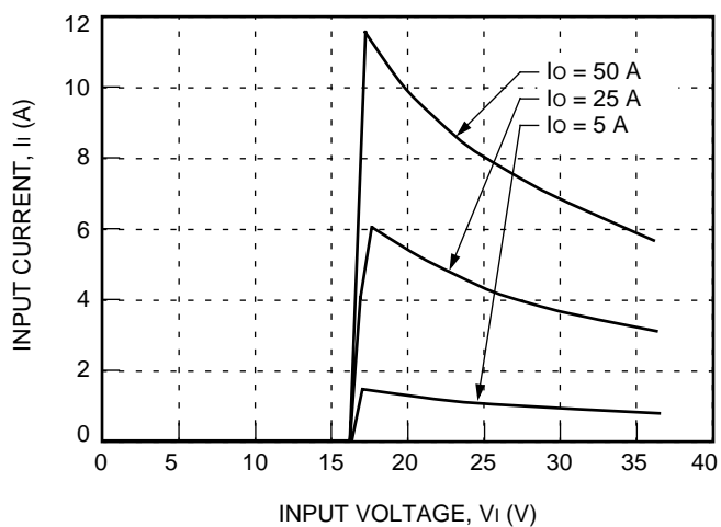
Figure 1. Typical FC250F1 Input Characteristics at Room Temperature
