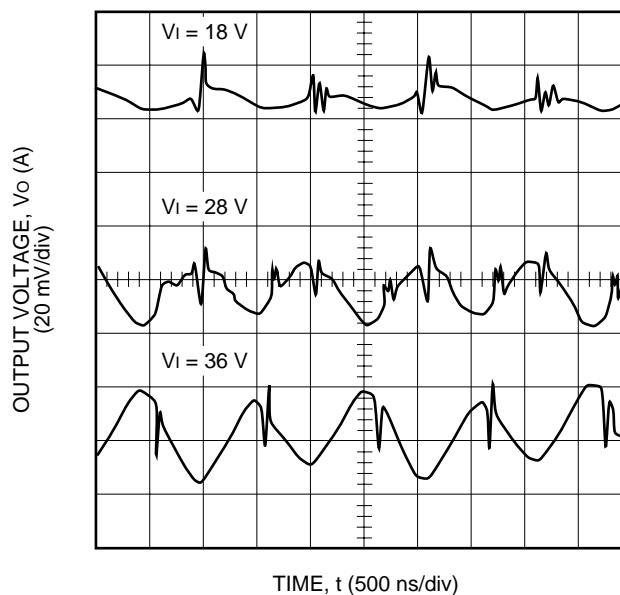
Figure 4. Typical FC250F1 Output Ripple Voltage at Room Temperature and 50 A Output
