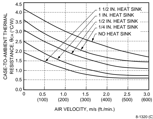
Figure 22. Case-to-Ambient Thermal Resistance Curves; Longitudinal Orientation
