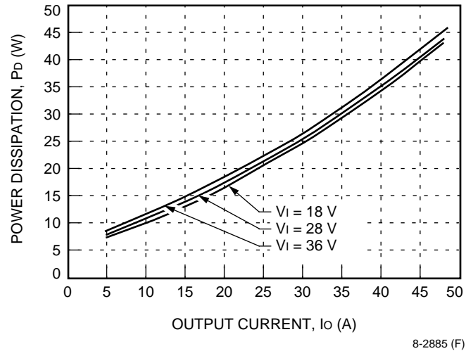
Figure 23. FC250F1 Power Dissipation vs. Output Current at 25 °C
