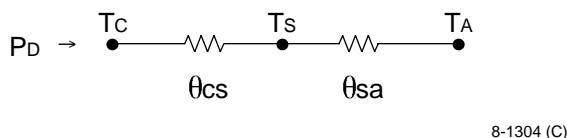
Figure 24. Resistance from Case-to-Sink and Sink-to-Ambient
