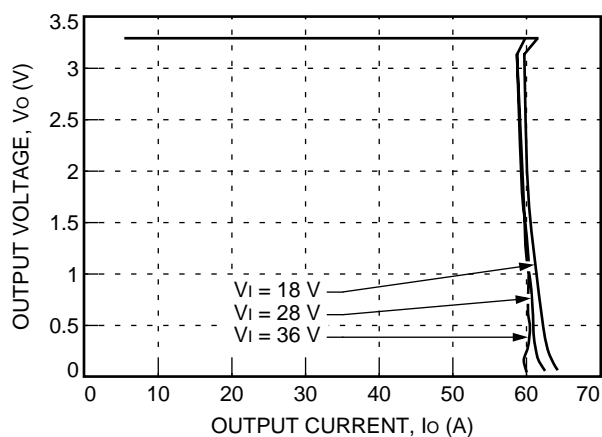
Figure 2. Typical FC250F1 Output Characteristics at Room Temperature
