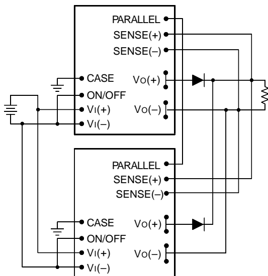
Figure 19. Wiring Configuration for Redundant Parallel Operation
