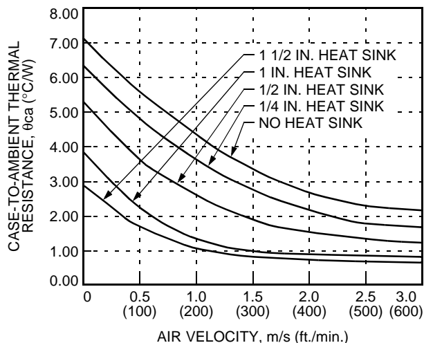
Figure 24. JAHW050A and JAHW075A Case-to-Ambient Thermal Resistance Curves; Either Orientation
