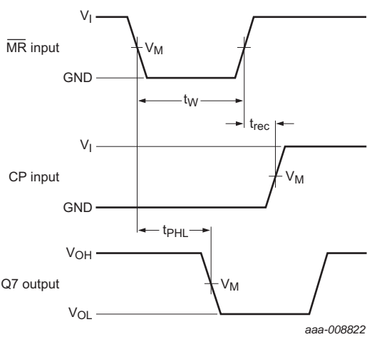
Measurement points are given in Table 8 . V_{OL} and V_{OH} are typical voltage output levels that occur with the output load.
