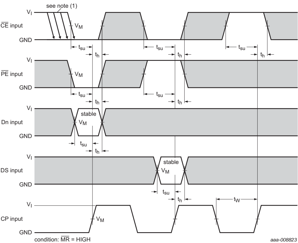
The shaded areas indicate when the input is permitted to change for predictable output performance Measurement points are given in Table 8 .
