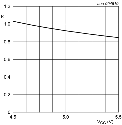
K-factor for 74HCT1G14-Q100
