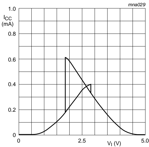
Fig 10. Typical 74HC1G14-Q100 transfer characteristics; V_{CC} = 4.5\text{ V}
