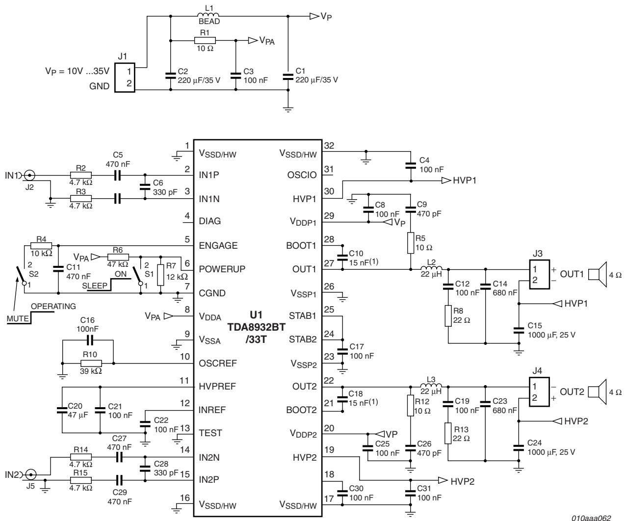
Fig 35. Schematic - version 3.00
