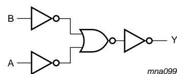
Fig 3. Logic diagram
